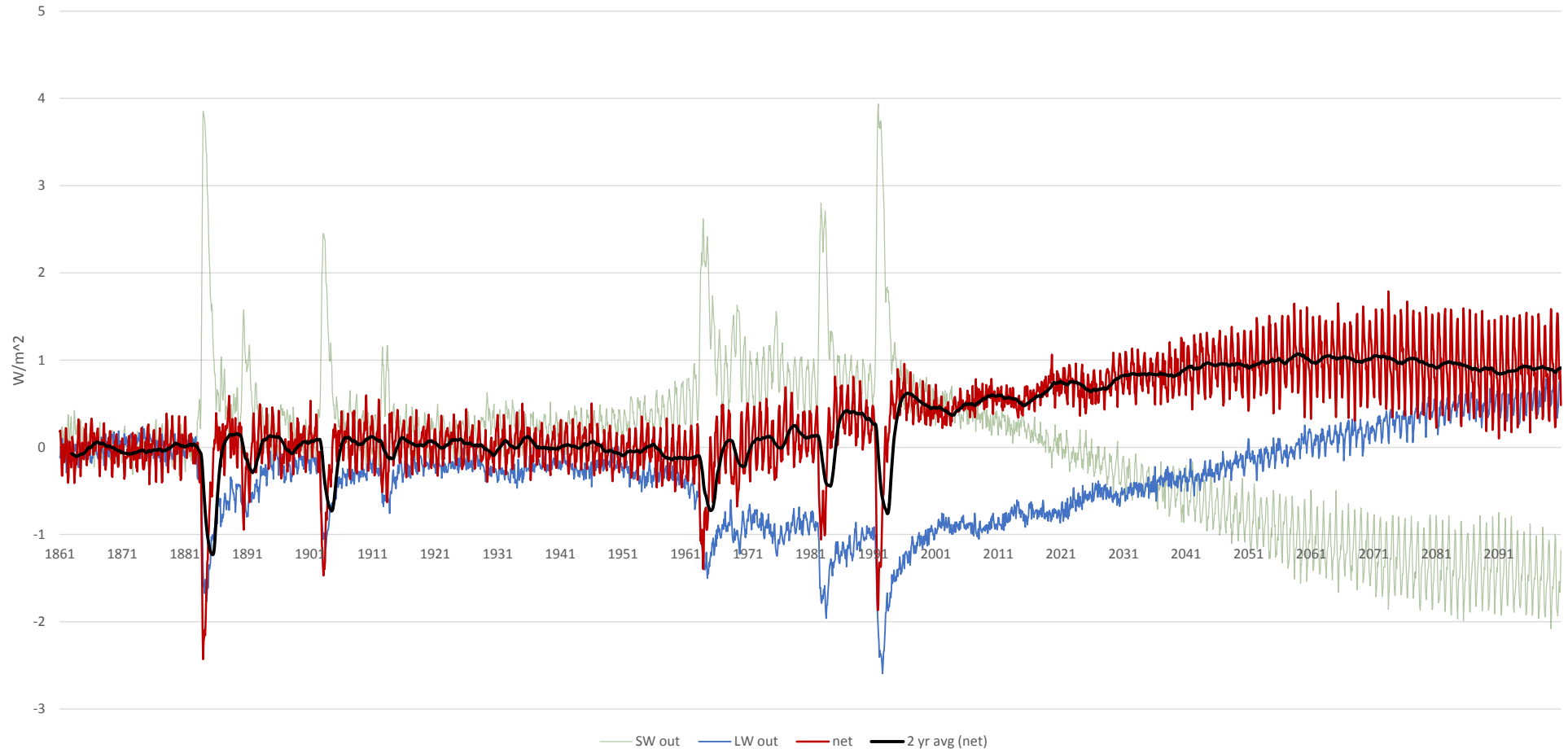
CMIP5 modmean rcp45, ToA radiation
