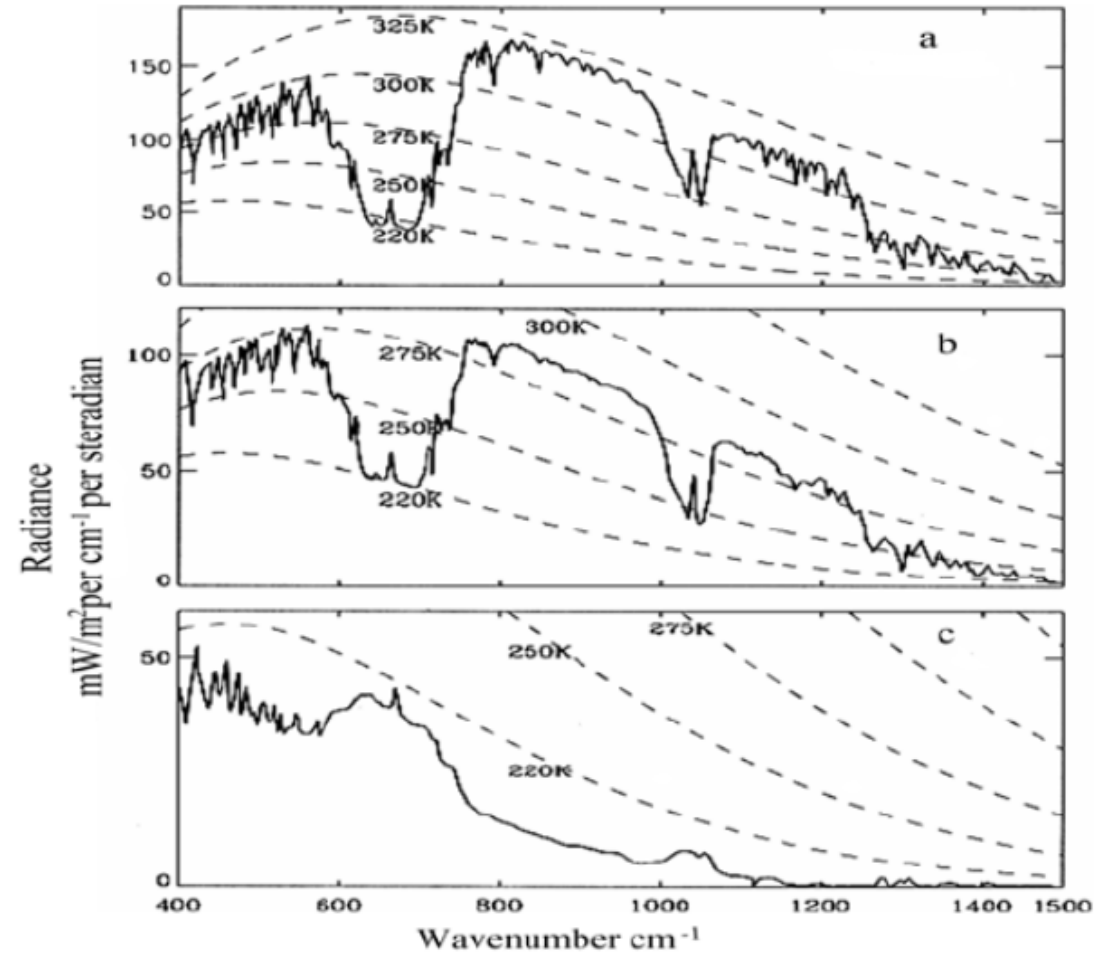
Fig. 16. Emission spectra of the Earth taken by the Nimbus 4 satellite. Spectrum (a) is measured over the Sahara Desert, spectrum (b) over the Mediterranean, and spectrum (c) over the Antarctic
