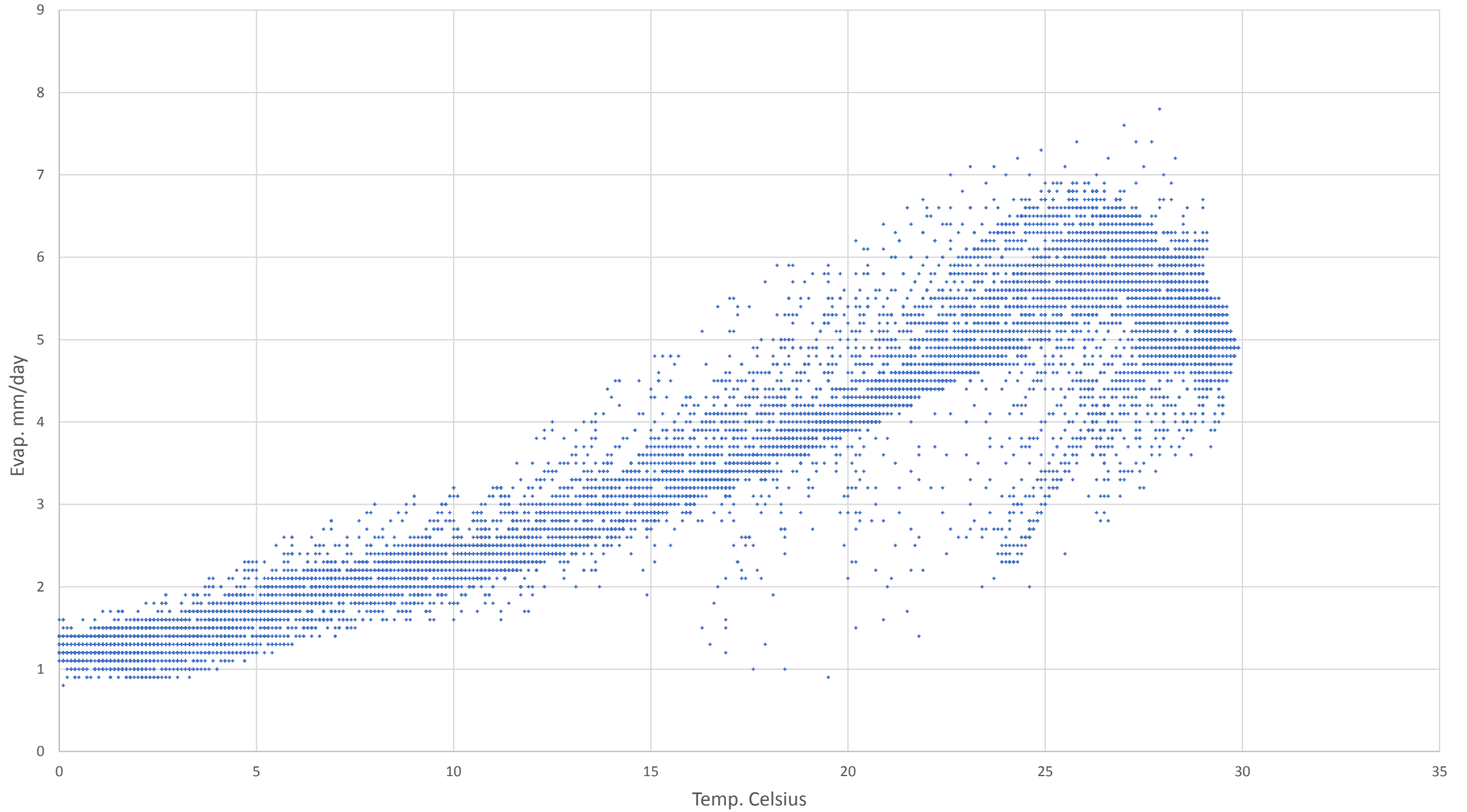
Evap vs. SST, SH annual, from JMA JRA-55 atlas
