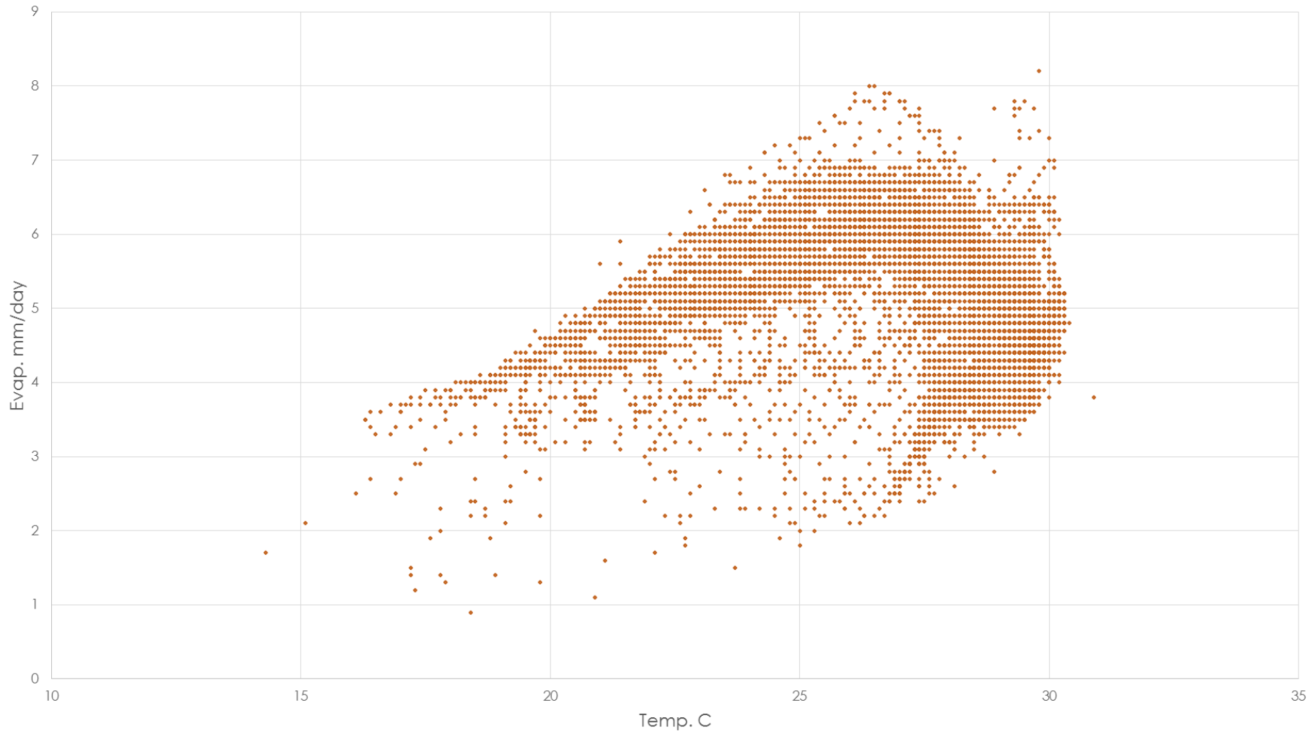
Evap vs. SST -30/30N April 1981-2010 from JMAs JRA-55 atlas
