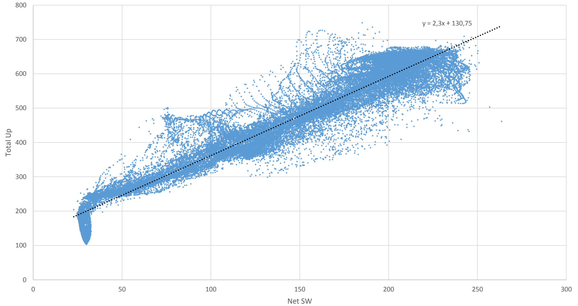
Absorbed Solar at the surface vs. LWup+Latent+Sensible, PERIOD : Annual; 30-year average (1981-2010) Data from JMAs JRA-55 atlas, 1,25x1,25 grid
